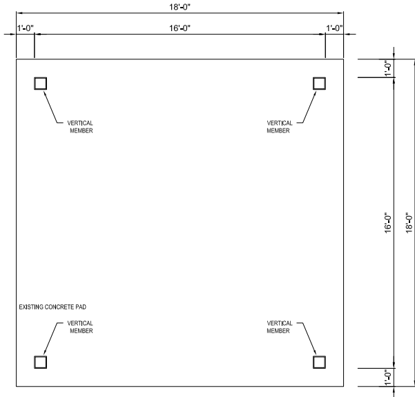
1 FLOOR PLAN
