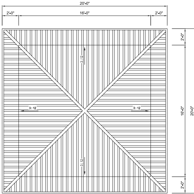
2 ROOF PLAN
