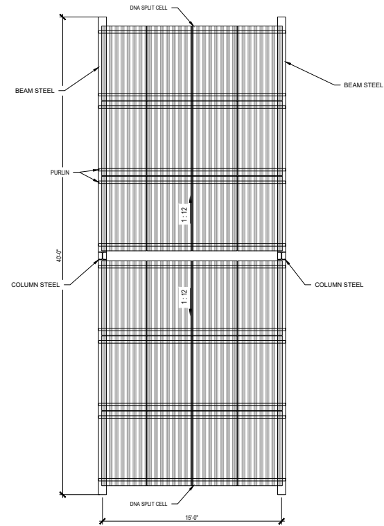
2 ROOF PLAN SCALE: 1/4"=1'-0"
