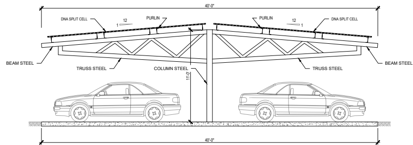
3 SIDE ELEVATION SCALE: 1/4"=1'-0"
